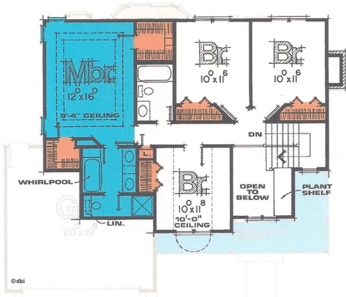
2nd Floor Plan (927 S.Q.)
