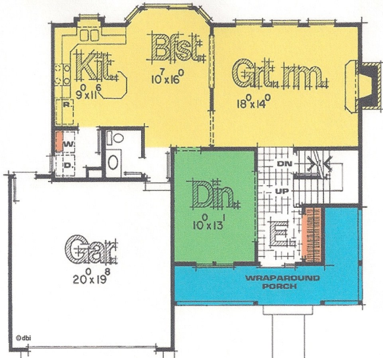
1st Floor Plan (919 S.Q.)
