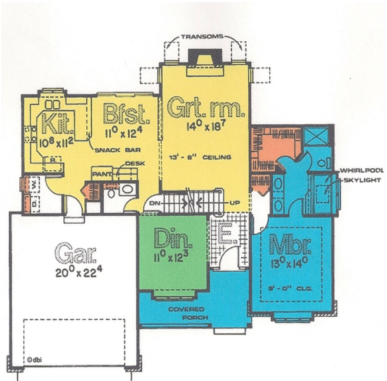
1st Floor Plan (1297 S.Q.)
