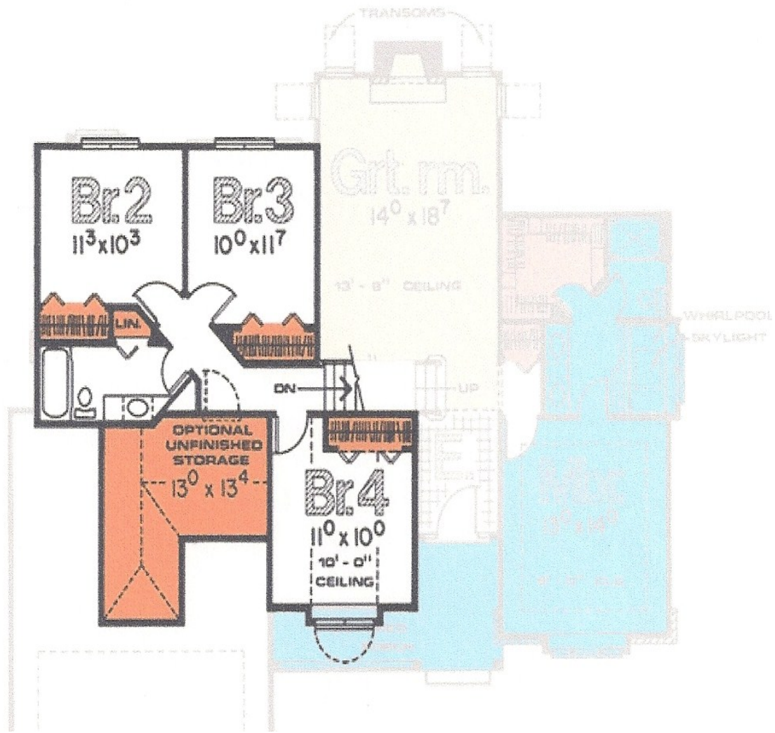
2nd Floor Plan (588 S.Q.)
